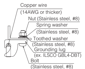
Fig. 5 Grounding method #3
