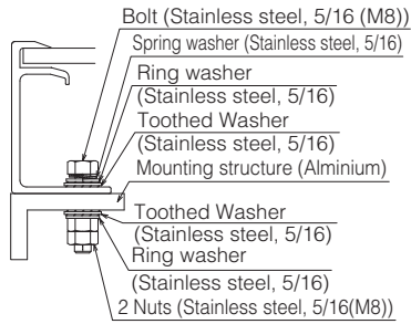
Fig. 6 Grounding method #4
