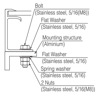
Fig. 1 Mounting of module
