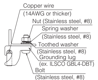
Fig. 5 Grounding method #3
